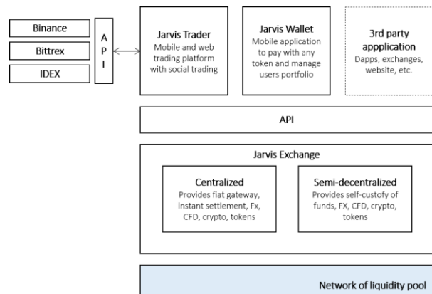
Figure 2. Applications layer.
